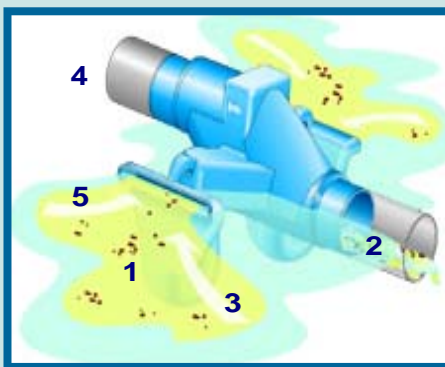
3P Overflow Siphon DN100-Steel Bars Rodent Barrier Art No. 4000215 Basic overflow with steel bars to keep out rodents.
