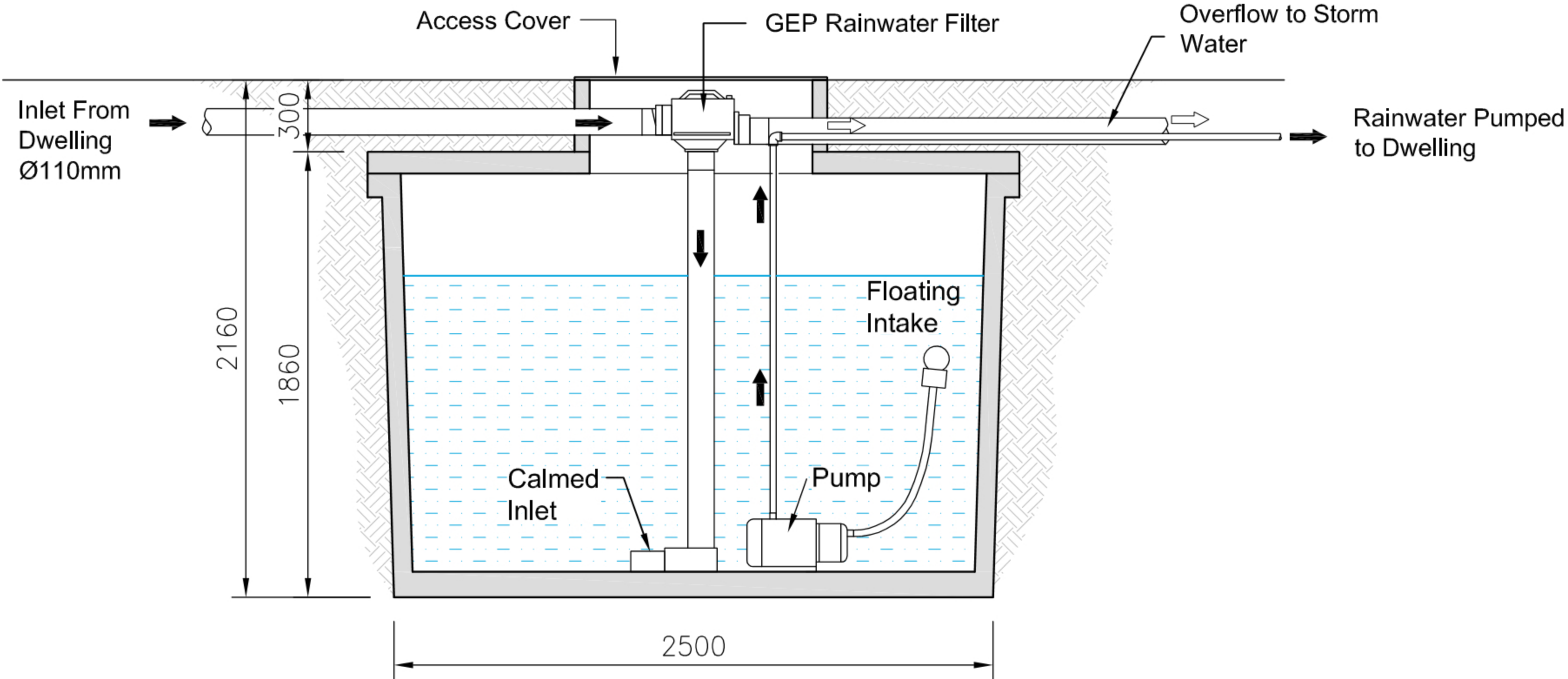
Section View
