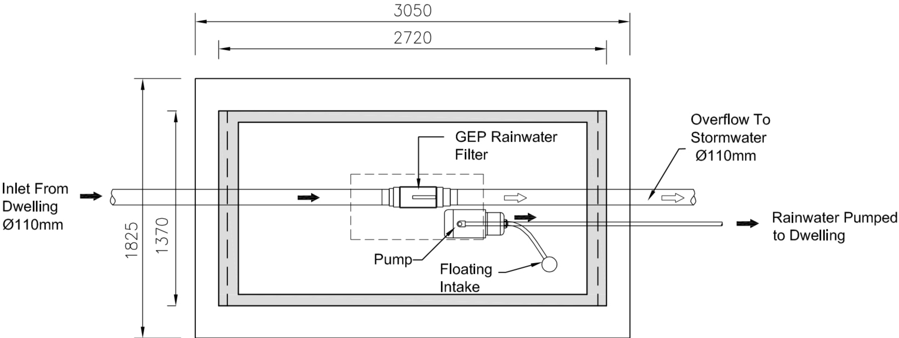
Plan View
