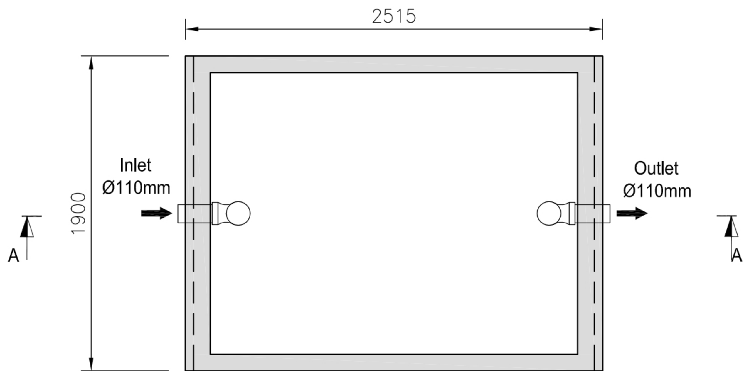
Plan View
