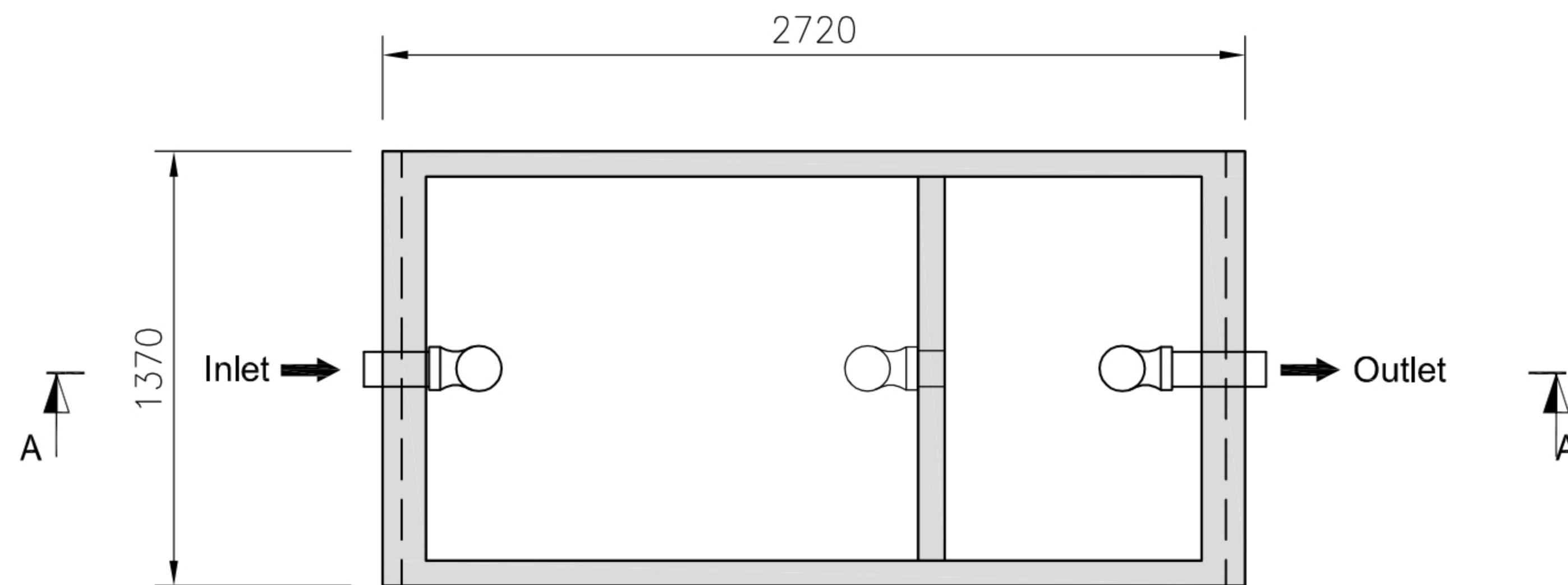
Plan View
