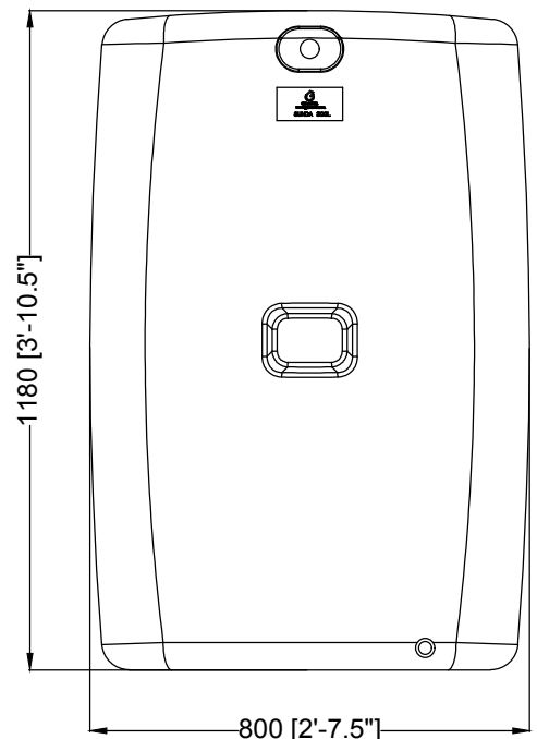
Hinteransicht View from back Vista de atrás Vue arrière
