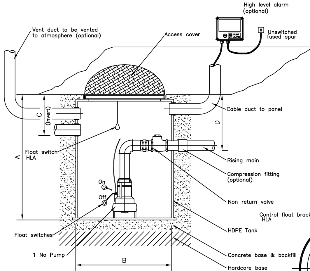
SIDE ELEVATION
